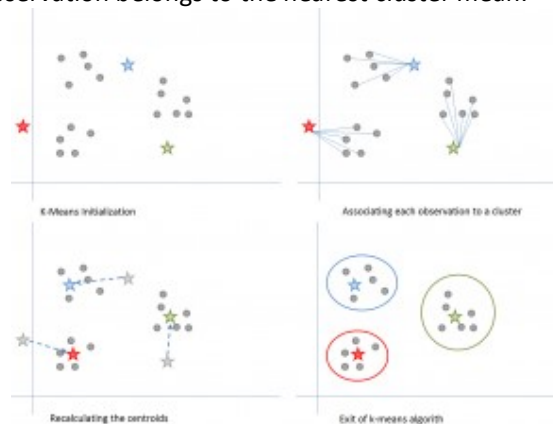
Steps of the K-means algorithm(source)
