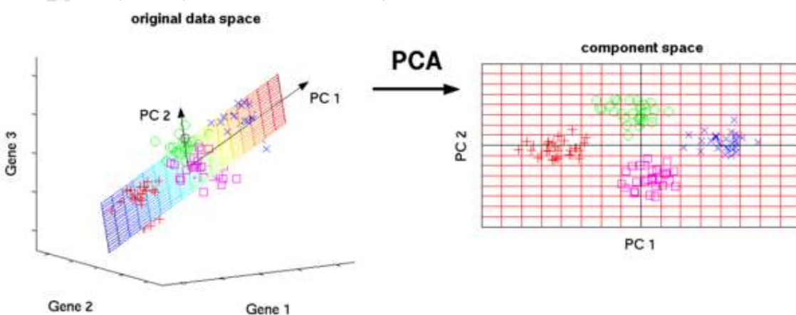
Principal Component Analysis
